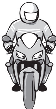
Rider countersteers.
